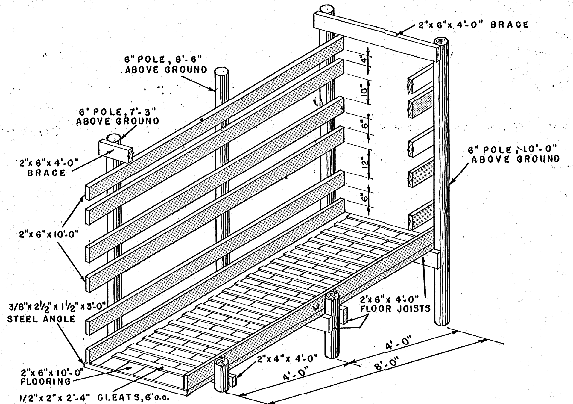
STATIONARY LOADING CHUTE
