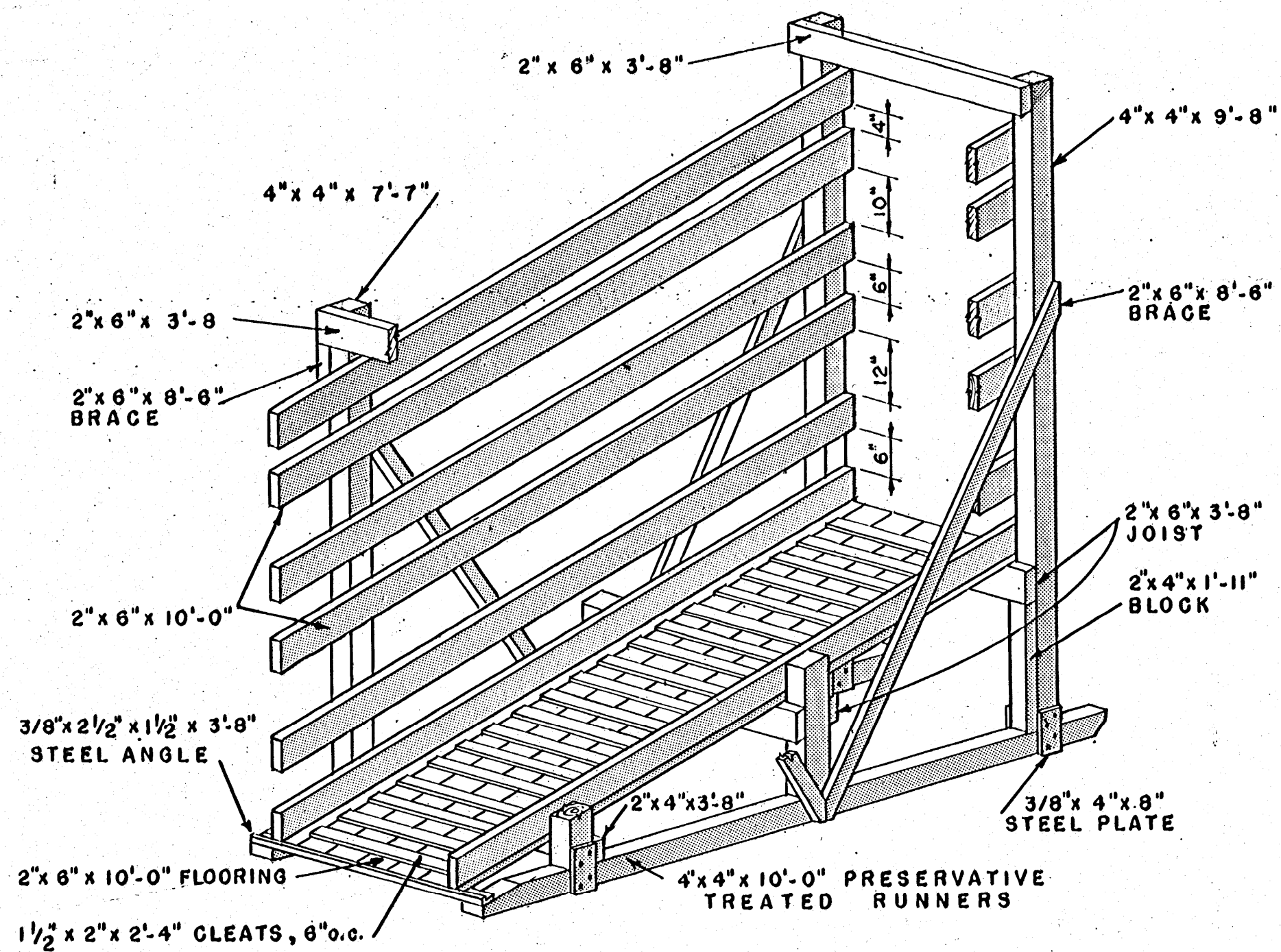
PORTABLE LOADING CHUTE
