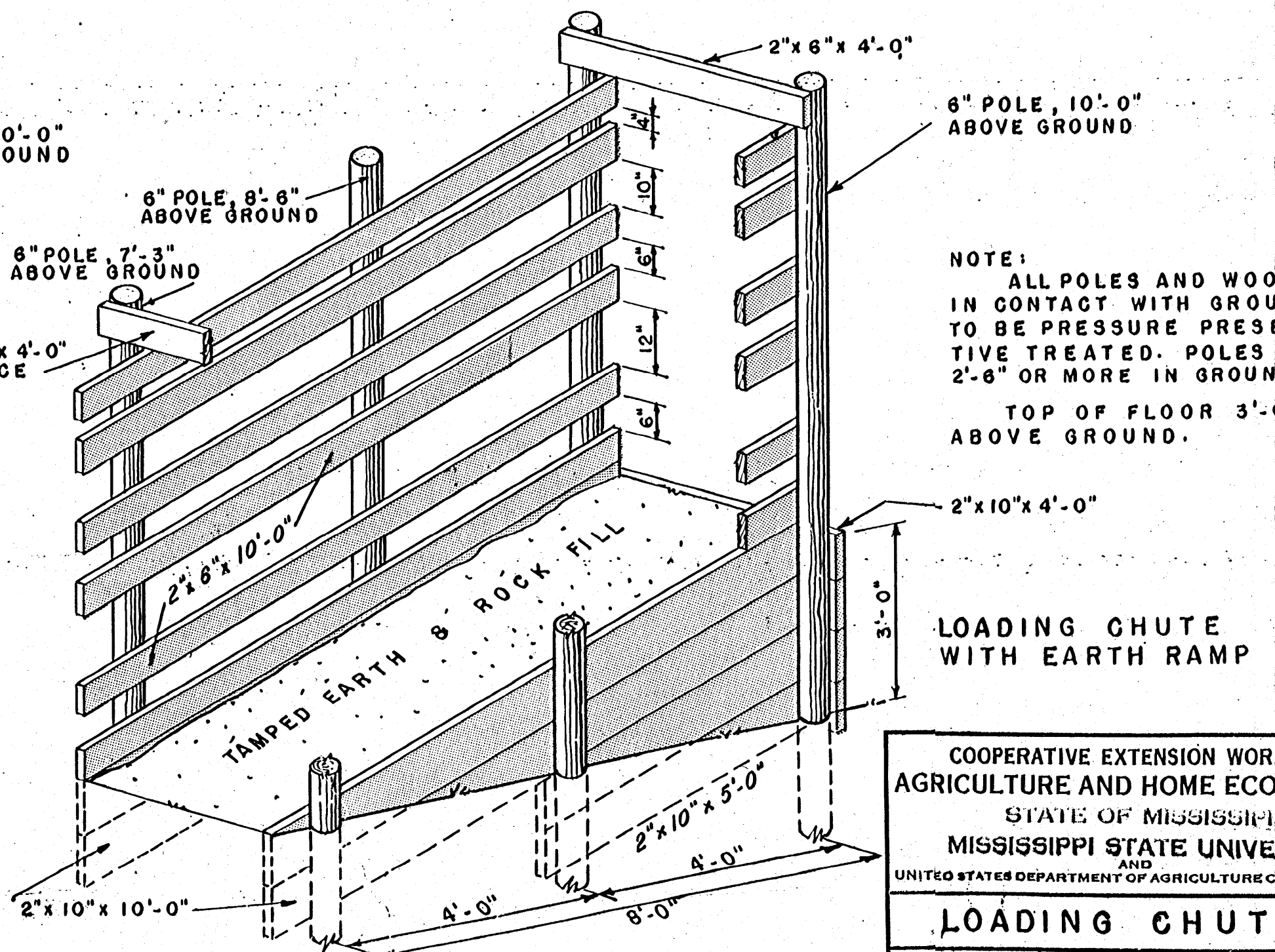
STATIONARY LOADING CHUTE
