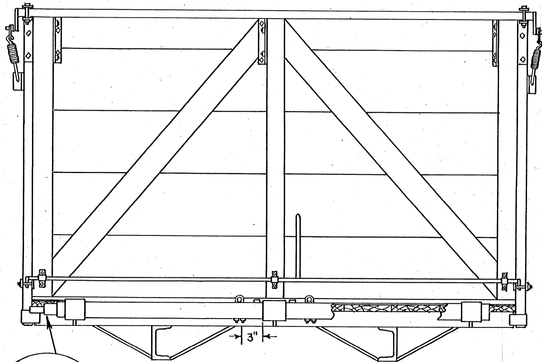
REAR VIEW
