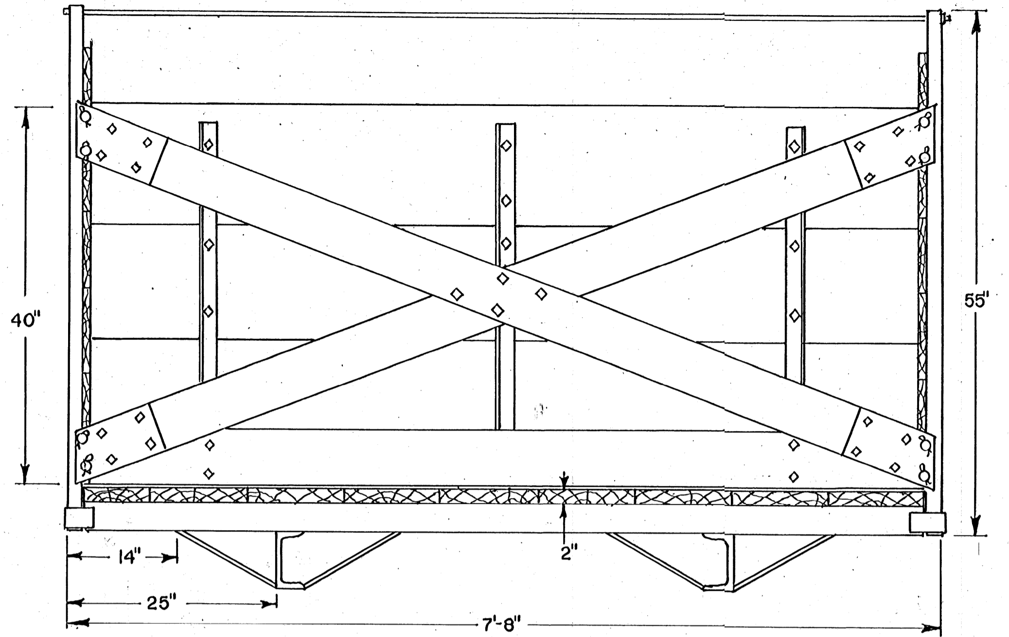
FRONT VIEW
