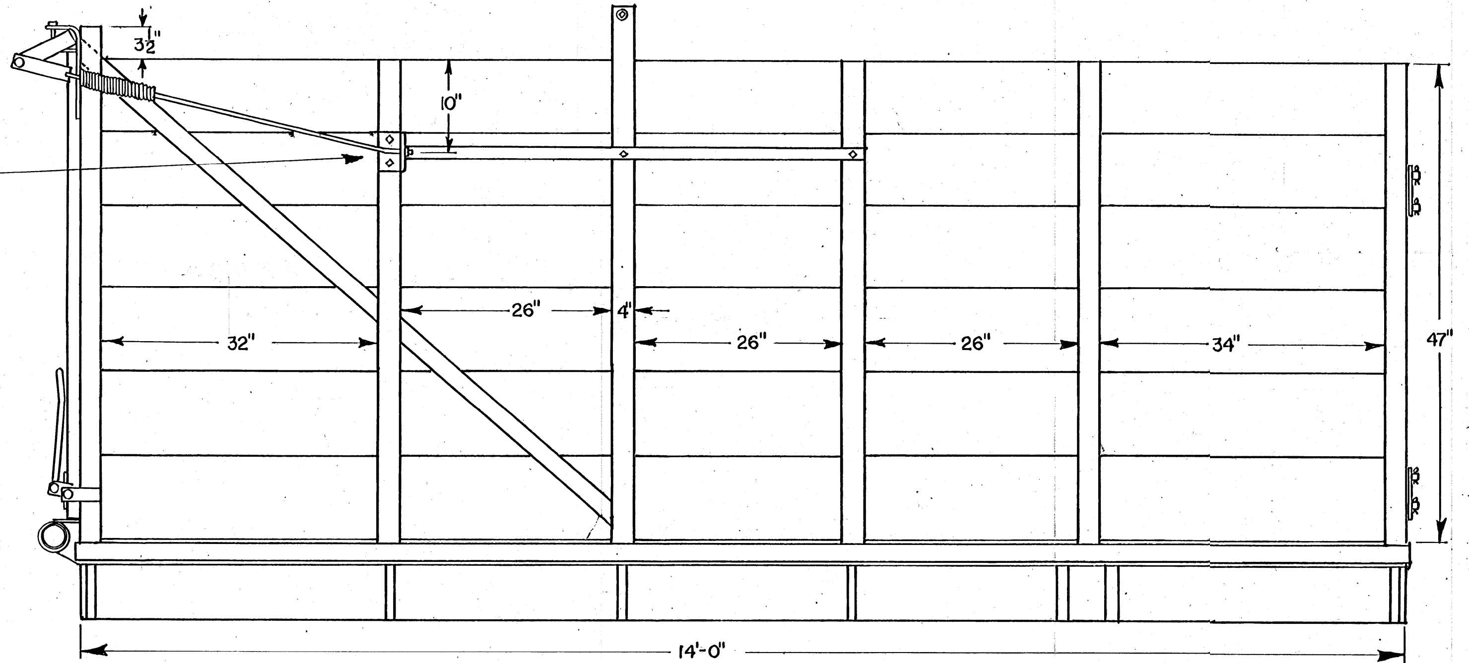
SIDE VIEW
